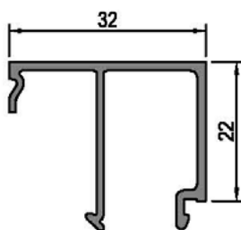
Junquillo 32 mm 40532
